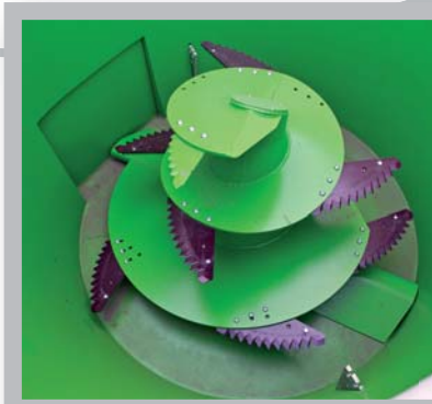
Heavy duty single auger equipped with high resistance toothed knives. Efficient design able to handle wet and dry stuff.
